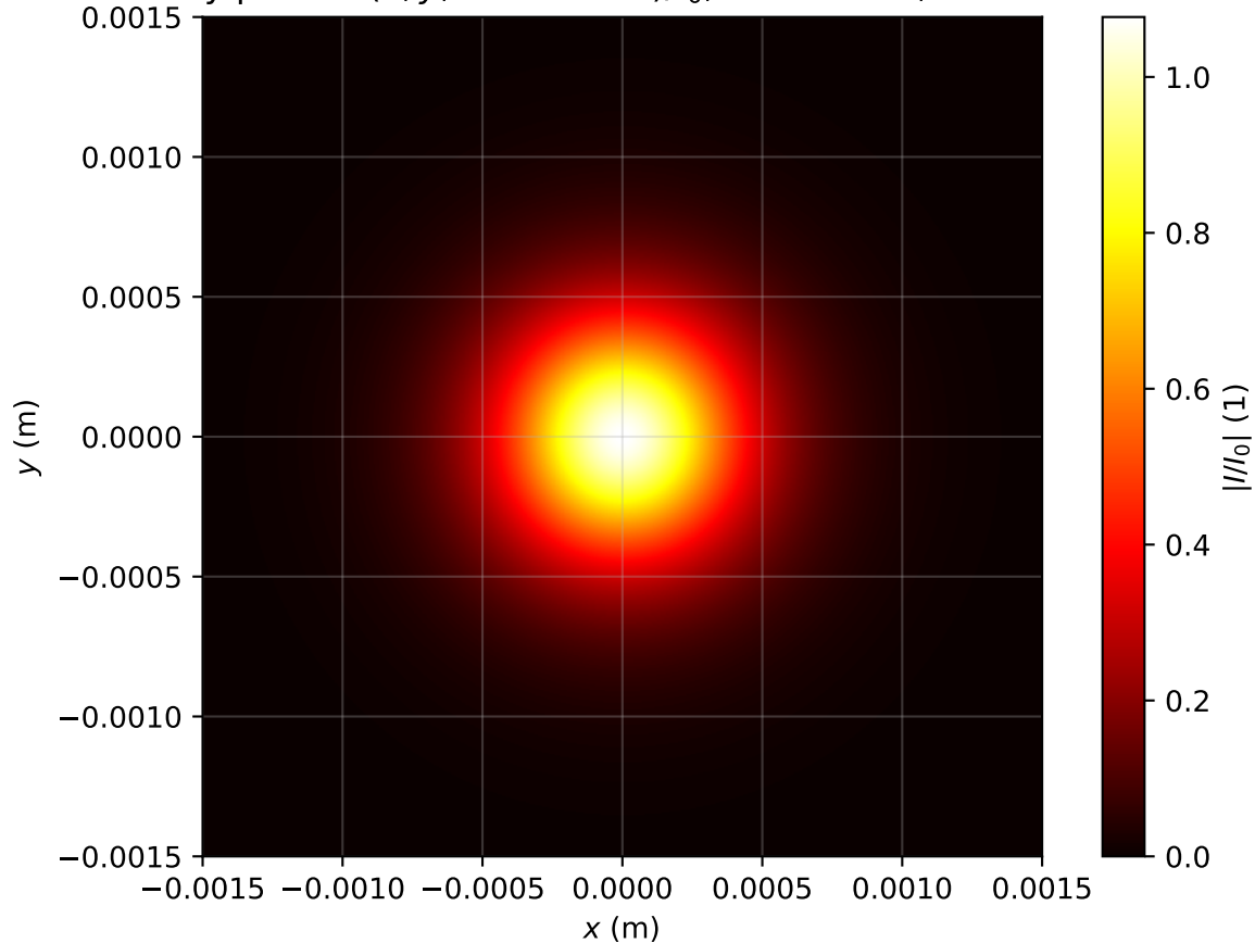
Intensity profile I(x, y, z = 1.433m)/I_0 , P_{in}=0.6P_{cr} , artificial time
